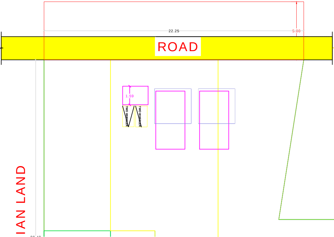
GROUND FLOOR RESIDENTIAL PLAN
