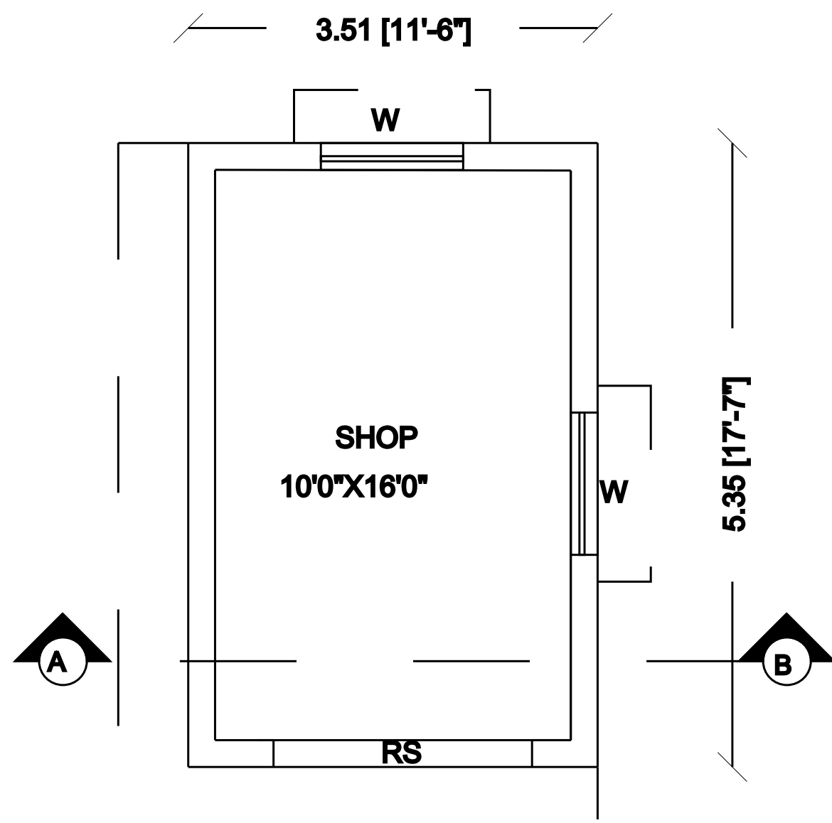
PLAN
