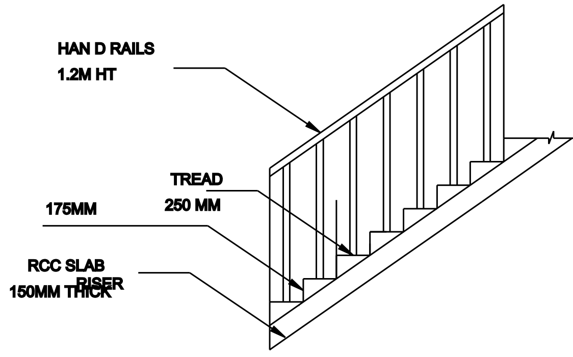
STAIRCASE DETAILS
