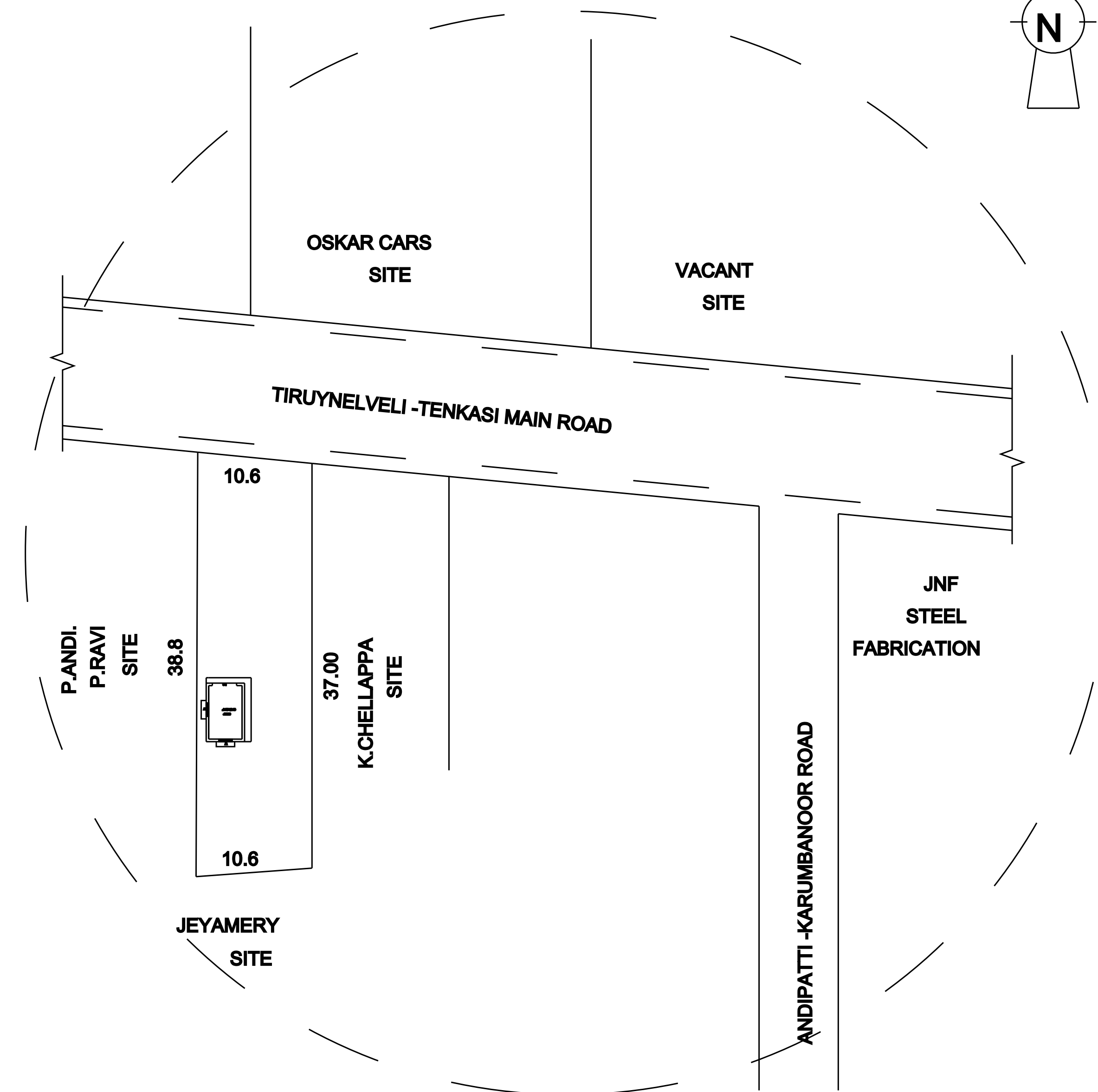
KEY PLAN
