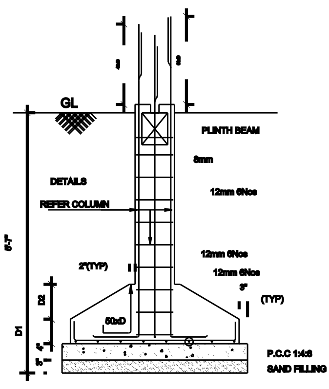
FOUNDATION DETAILS
