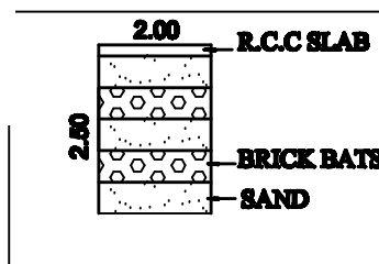
RAIN WATER HARVEST PIT PLAN
