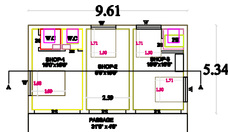
1D FLOOR PLAN
