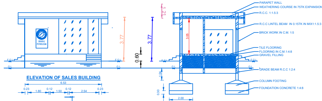
SECTION ON AA OF SALES BUILDING
