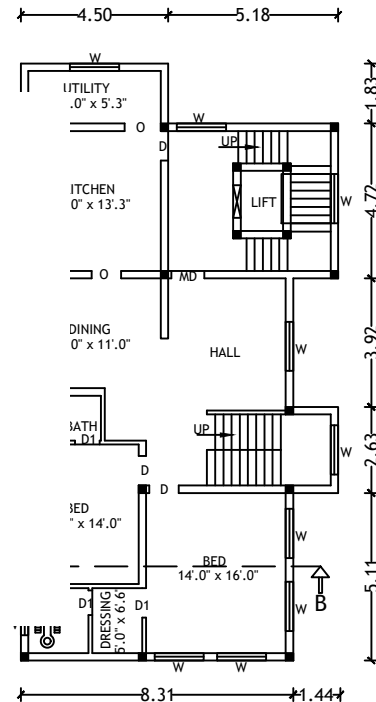
PLAN FIRST FLOOR
