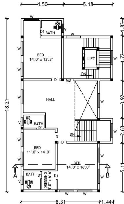
PLAN SECOND FLOOR
