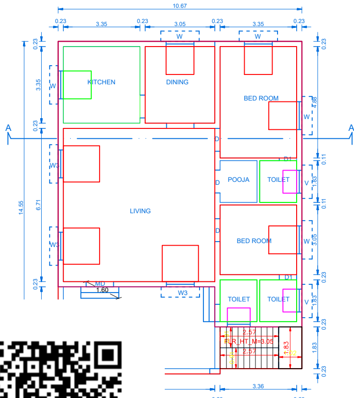
D FLOOR
