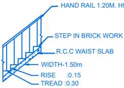
STAIR DETAIL
