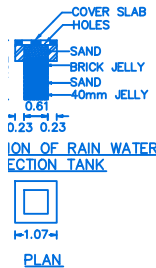
RAIN WATER COLLECTION TANK
