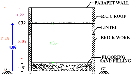
"SECTION "AB"
