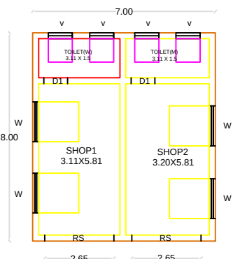
PROPOSED FF PLAN
