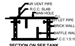
SECTION ON SEP. TANK
