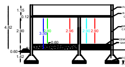
SECTION ON "AB"
