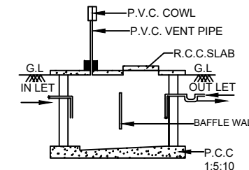
SEC. OF SEPTIC TANK
