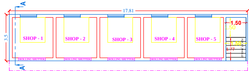
PLAN - FIRST FLOOR ( PROPOSED )
