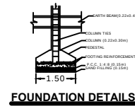
FOUNDATION DETAILS
