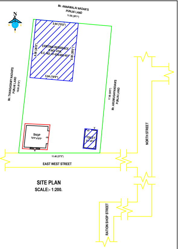
LOCATION MAP
