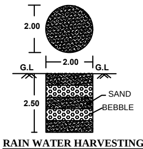
ALL DIMENSION ARE IN METRE SCALE 1:100
