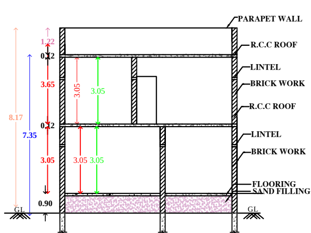
"SECTION "AB"
