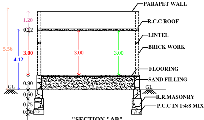
"SECTION "AB"
