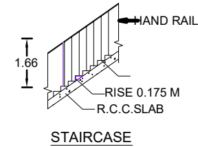
STAIRCASE
