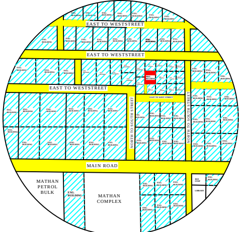
TOPO PLAN
