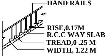
SECTION ON STAIR
