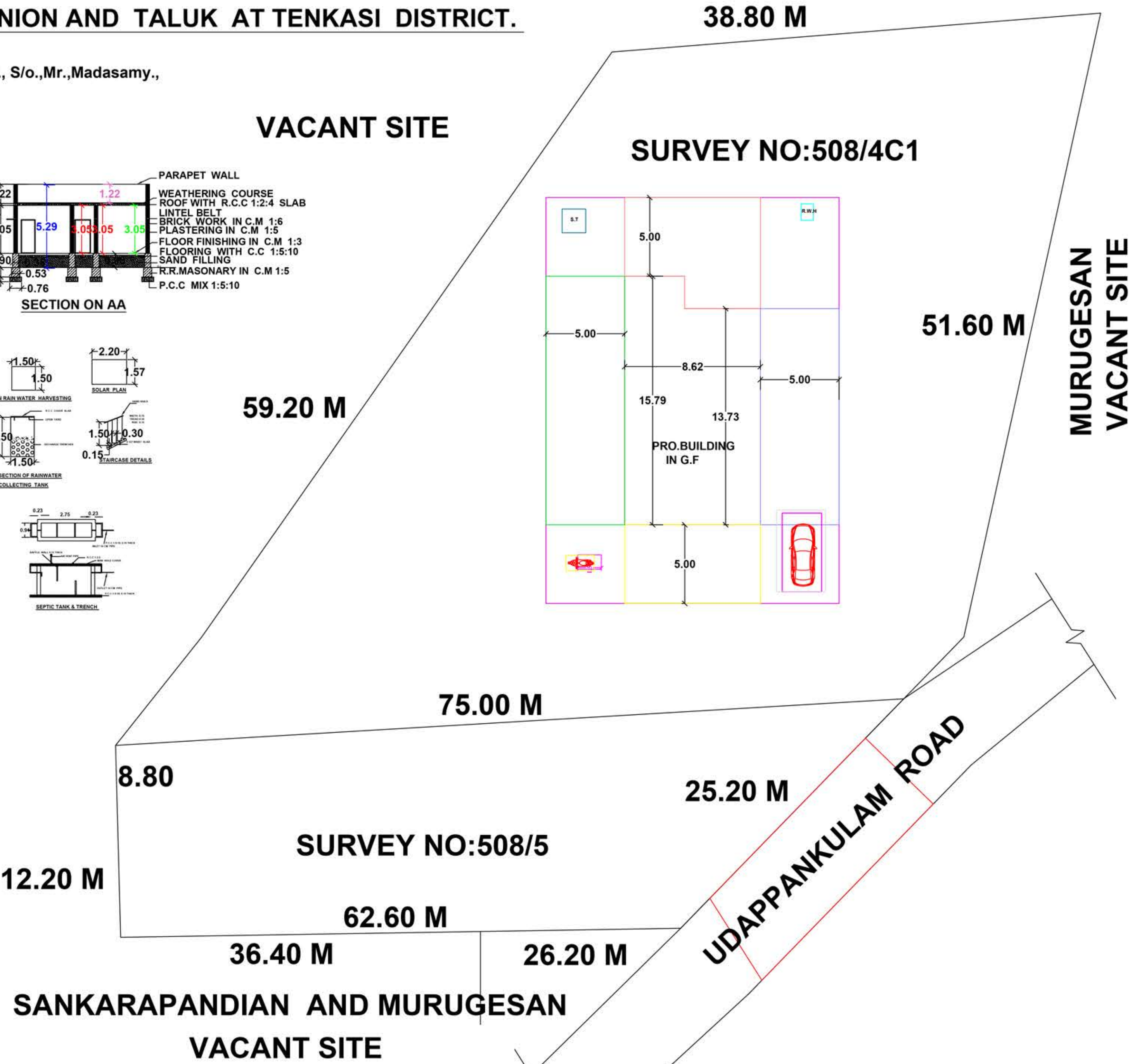
SITE PLAN
