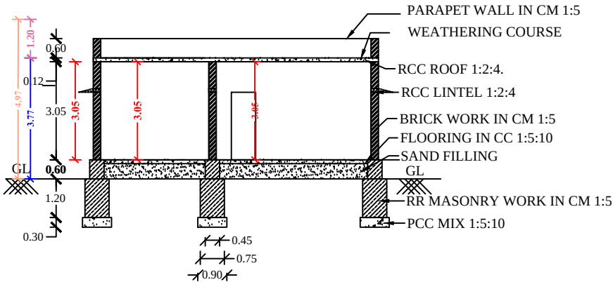
SECTION OF "BS"
