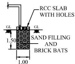
SECTION OF BS
