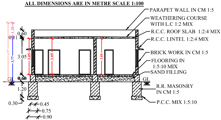
SECTION OF "AB"
