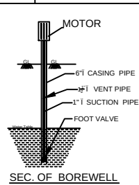
SEC. OF BOREWELL
