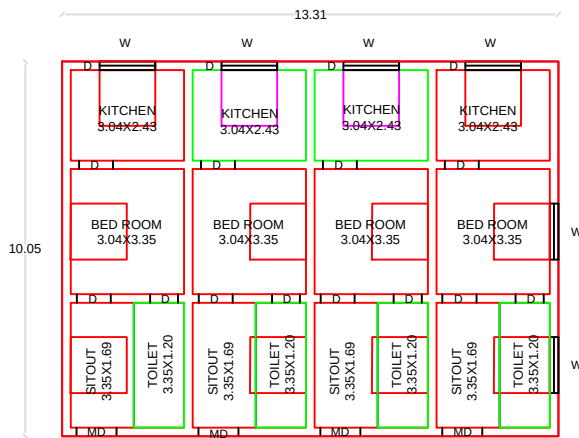
PROPOSED GF PLAN
