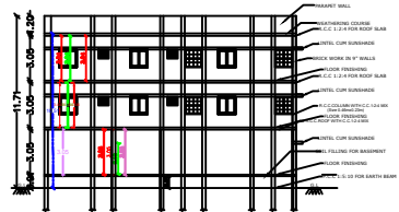
SECTION-AB
