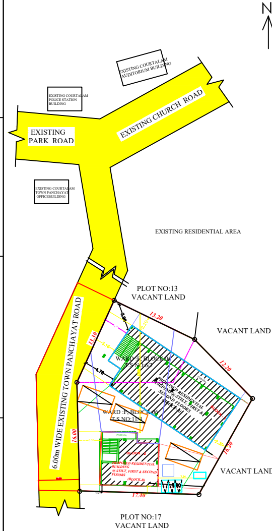
SITE PLAN
