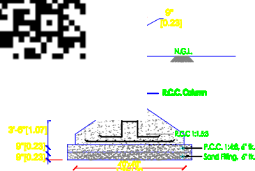
FOUNDATION DETAIL
