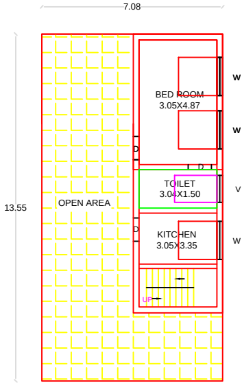
PROPOSED FF PLAN
