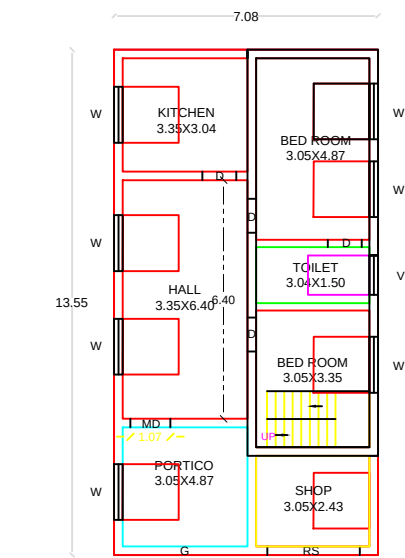
PROPOSED GF PLAN
