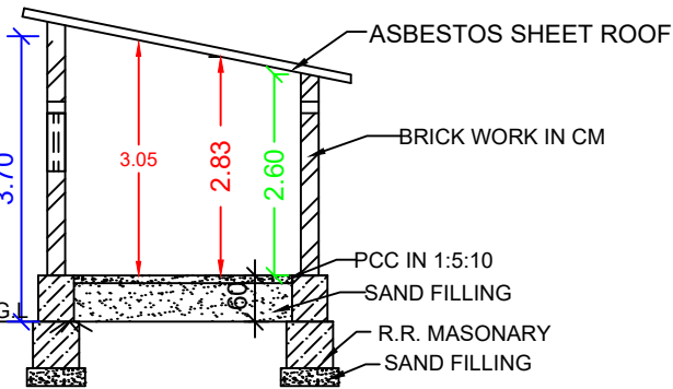
SECTION "AB"
