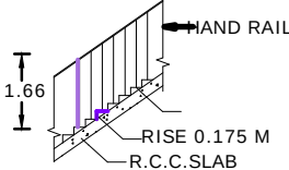
STAIRCASE
