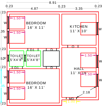
GROUND FLOOR RESIDENTIAL PLAN
