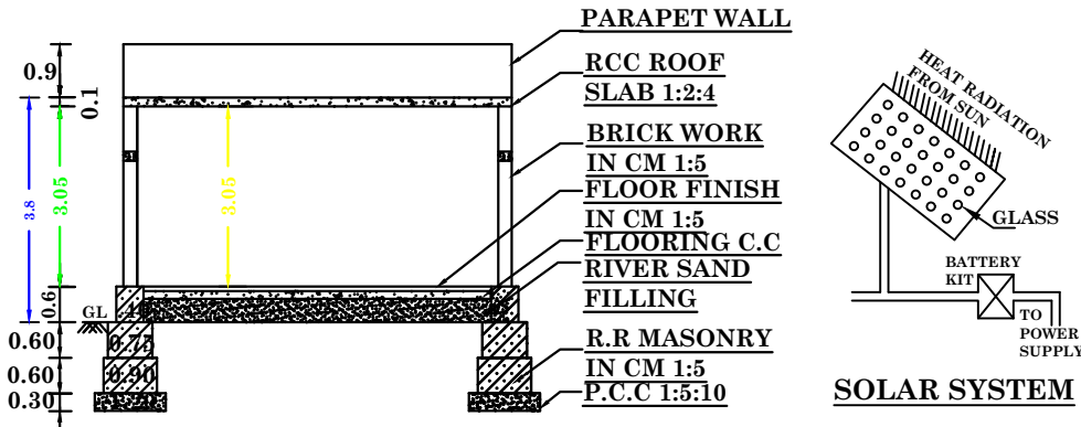
SECTION ON AA1
