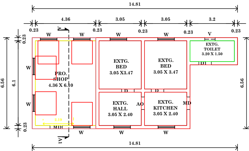
EXISTING AND PROPOSED GROUND FLOOR PLAN
