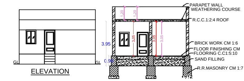
SECTION ON SV
