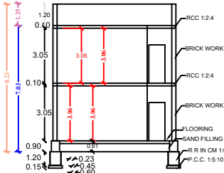
SECTION AB
