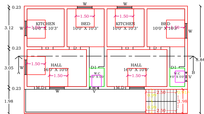
PRO-FIRST FLOOR
