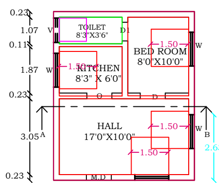
PLAN BLOCK - II
