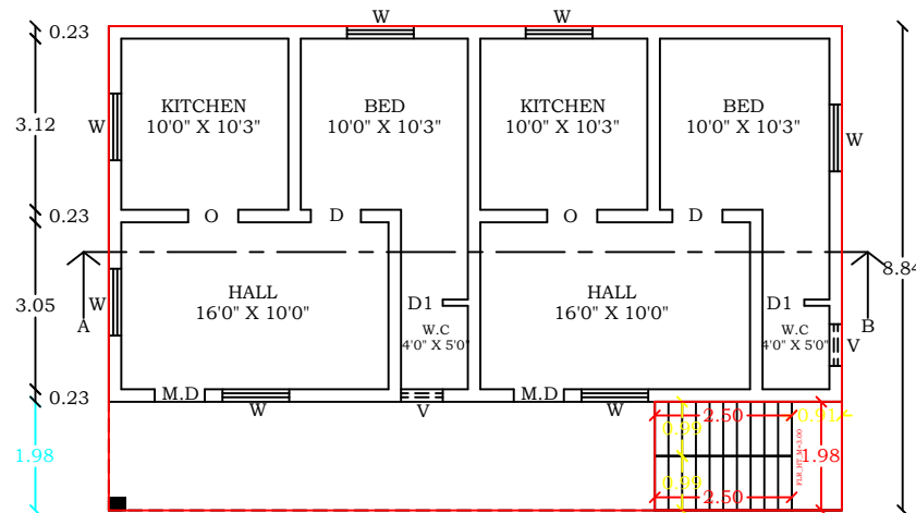
EXG.GROUND FLOOR
