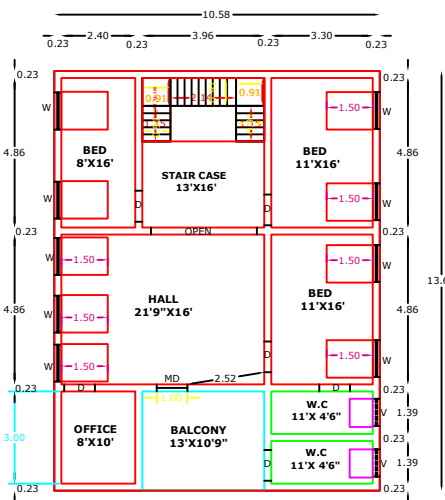
FIRST FLOOR RESIDENTIAL PLAN
