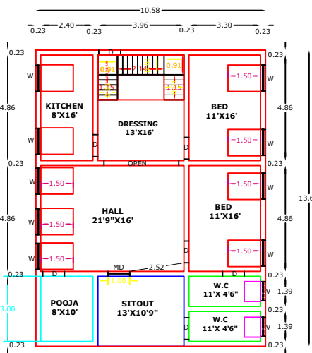
GROUND FLOOR RESIDENTIAL PLAN
