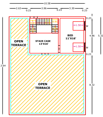
SECOND FLOOR RESIDENTIAL PLAN
