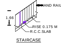
STAIRCASE
