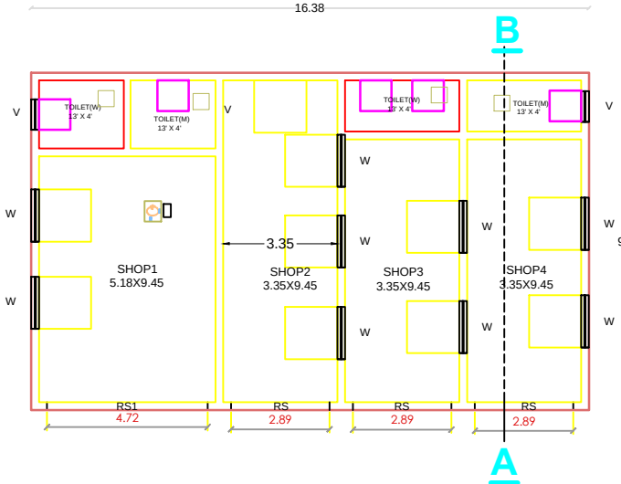
PROPOSED GF PLAN
