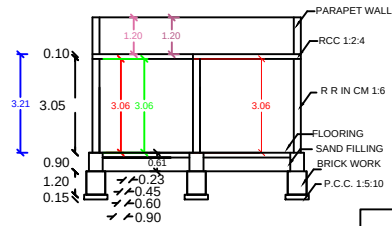
SECTION AB
