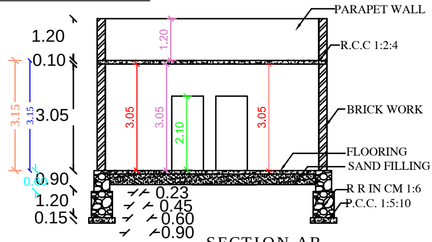
SECTION AB
