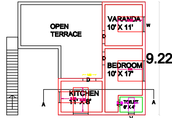
PROPOSED FIRST FLOOR
