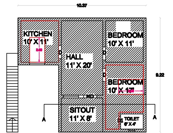
PROPOSED FIRST FLOOR
