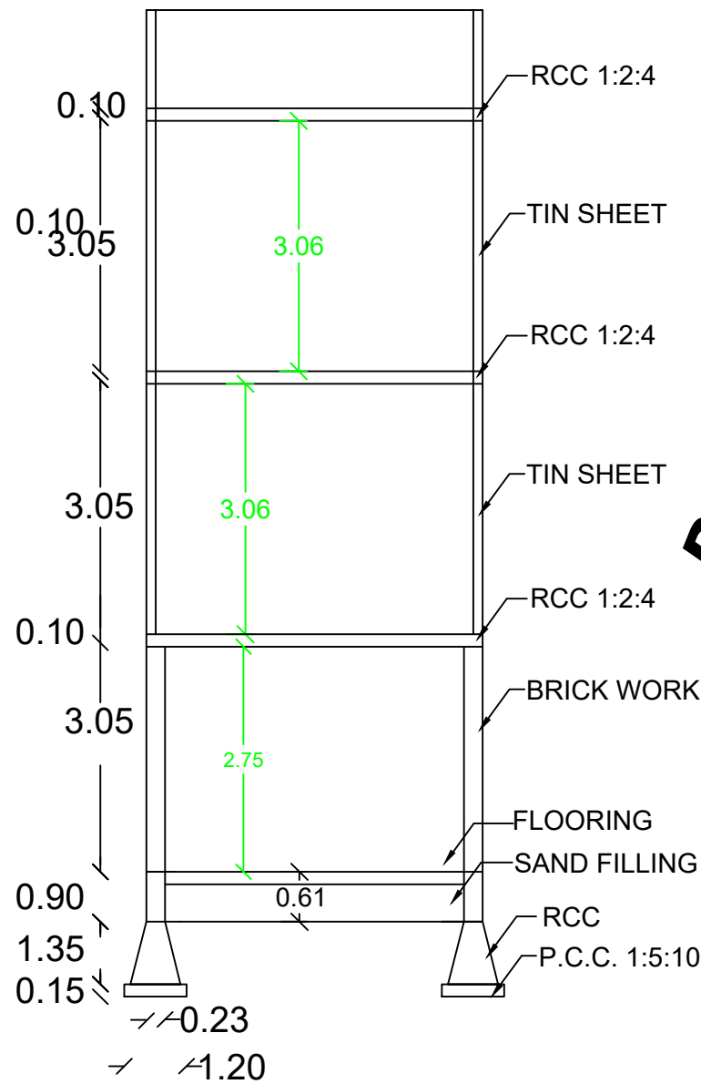
SECTION AB
