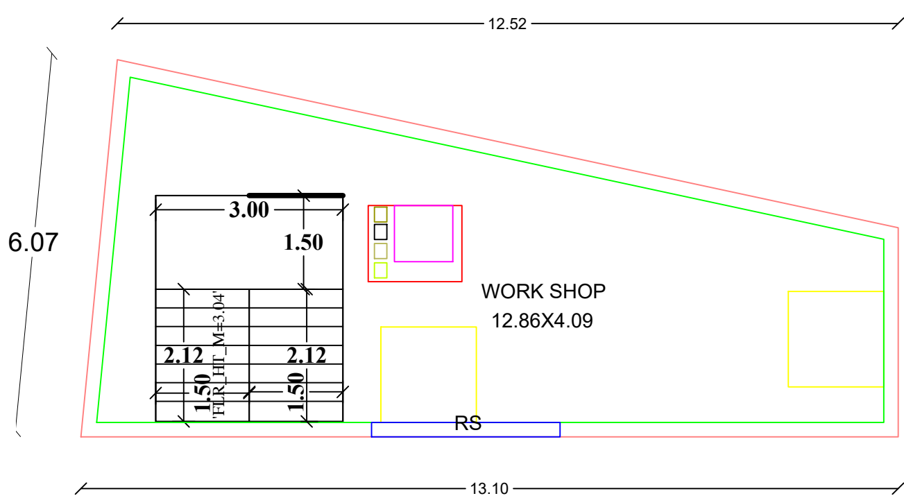
GROUND FLOOR PALN
