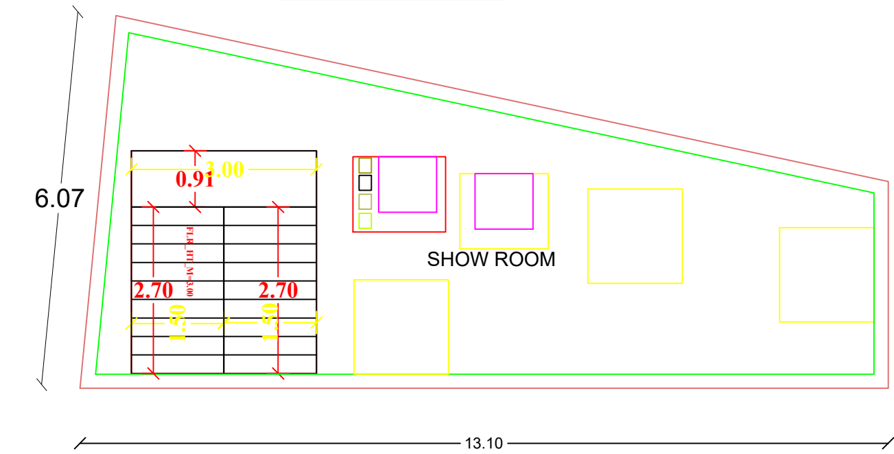
FIRST FLOOR PALN
