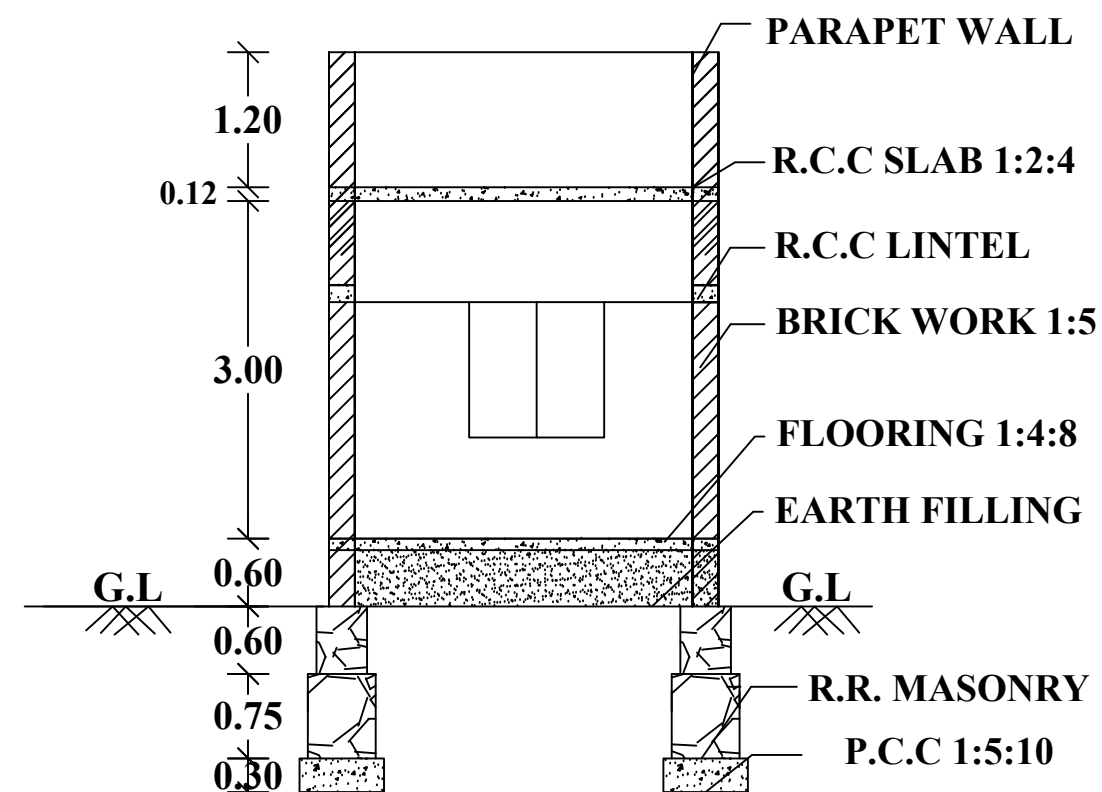
"SECTION "AB"
