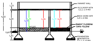
SECTION ON "AB"
