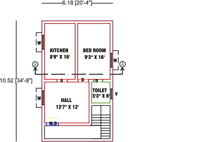
PROPOSED/ADDITIONAL FIRST FLOOR PLAN
