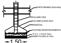
FOUNDATION DETAILS
