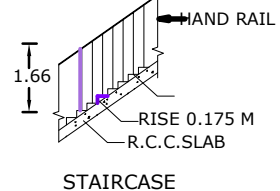
STAIRCASE
