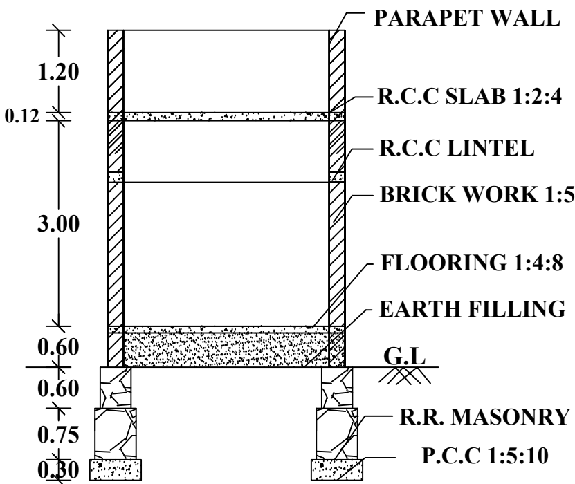
"SECTION "AB"
