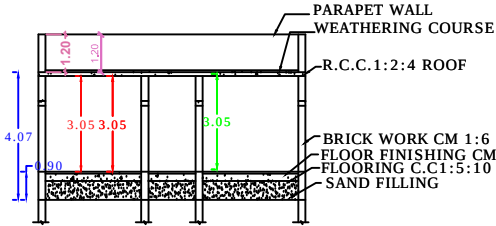
SECTION ON SV
