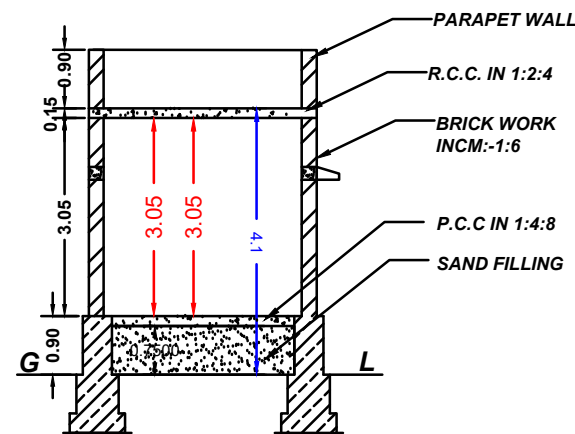
SECTION "AB"
