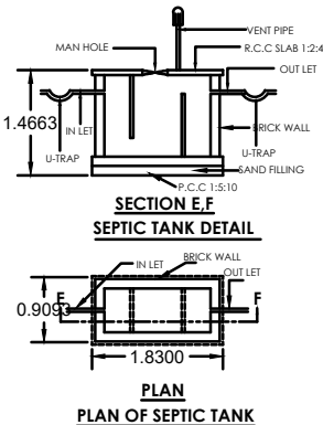
PLAN PLAN OF SEPTIC TANK
