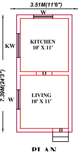
PLAN
