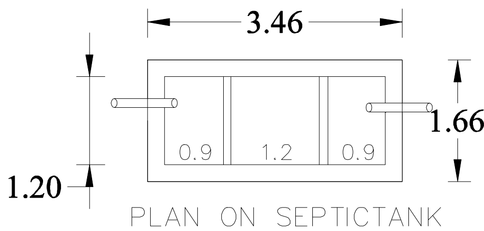
PLAN ON SEPTICTANK
