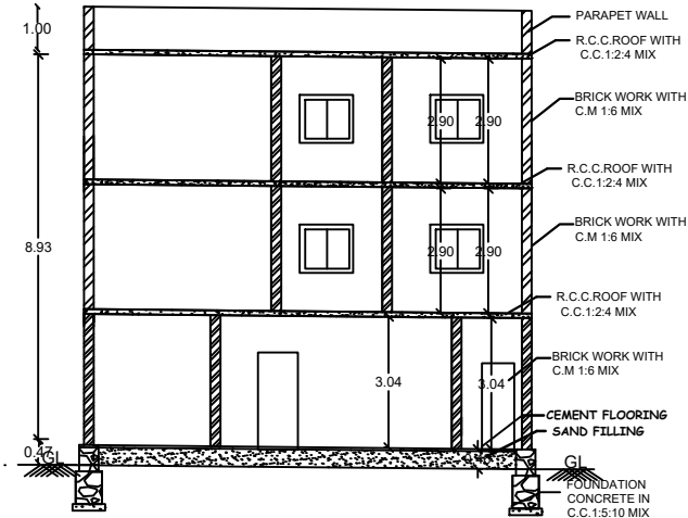
SECTION AB
