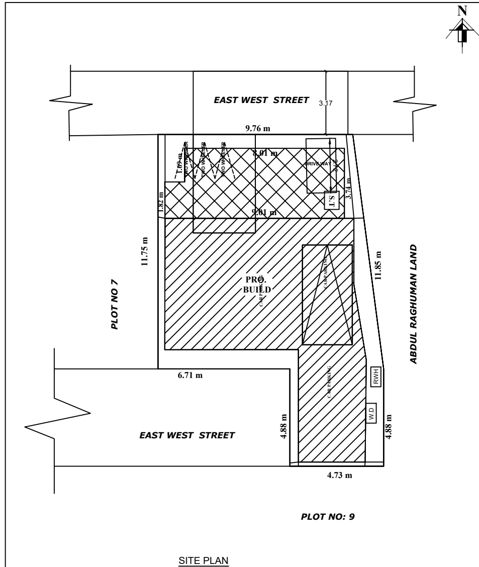
SITE PLAN
