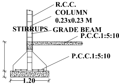
COLUMN DETAIL
