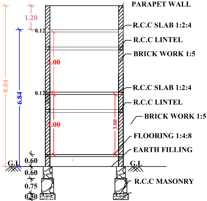
"SECTION 'AB'"
