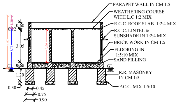
SECTION OF "AB"
